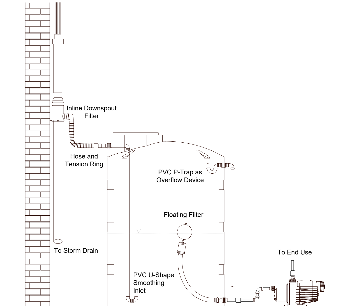
Aboveground System with Inline Downspout Filter and Jet Pump
