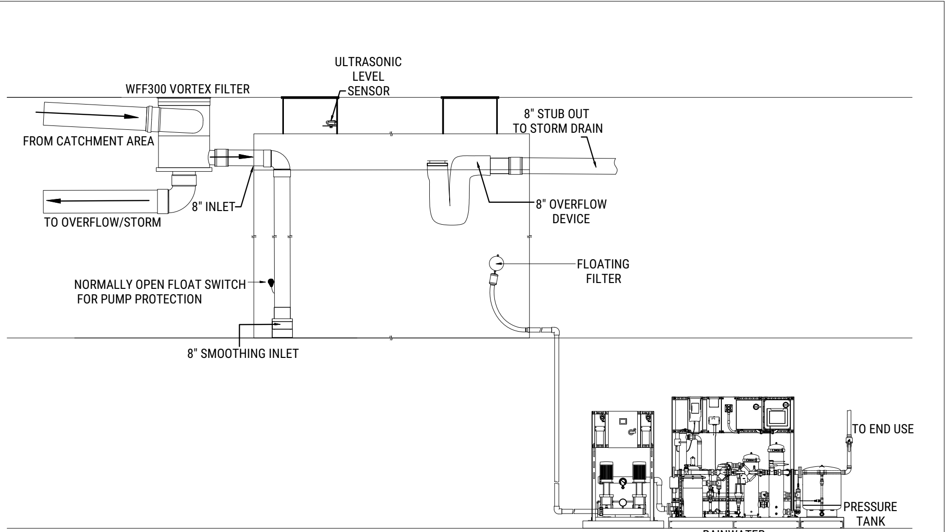
RAINWATER FILTRATION SKID (SHOWN WITH DOMESTIC)
