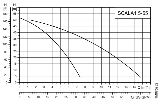
Fig. Performance curves, SCALA1 5-55 twin
